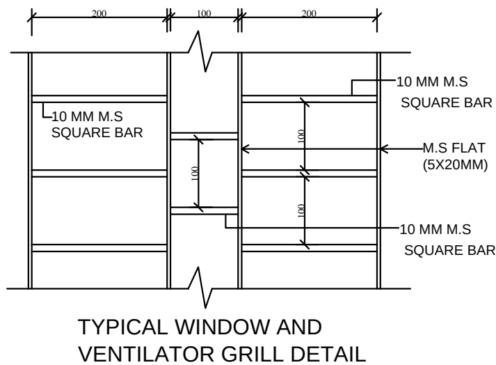
WINDOW TYPE W1V1
