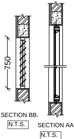
WINDOW TYPE WV
